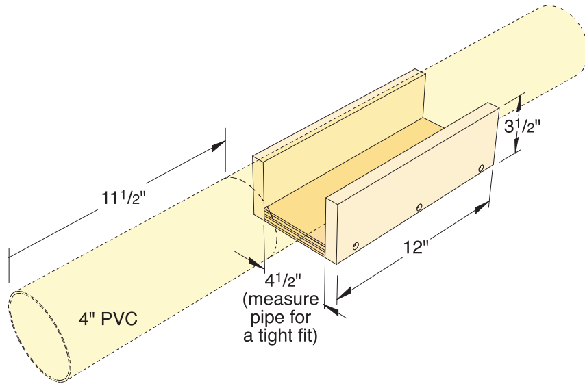
PVC CUTTING JIG
